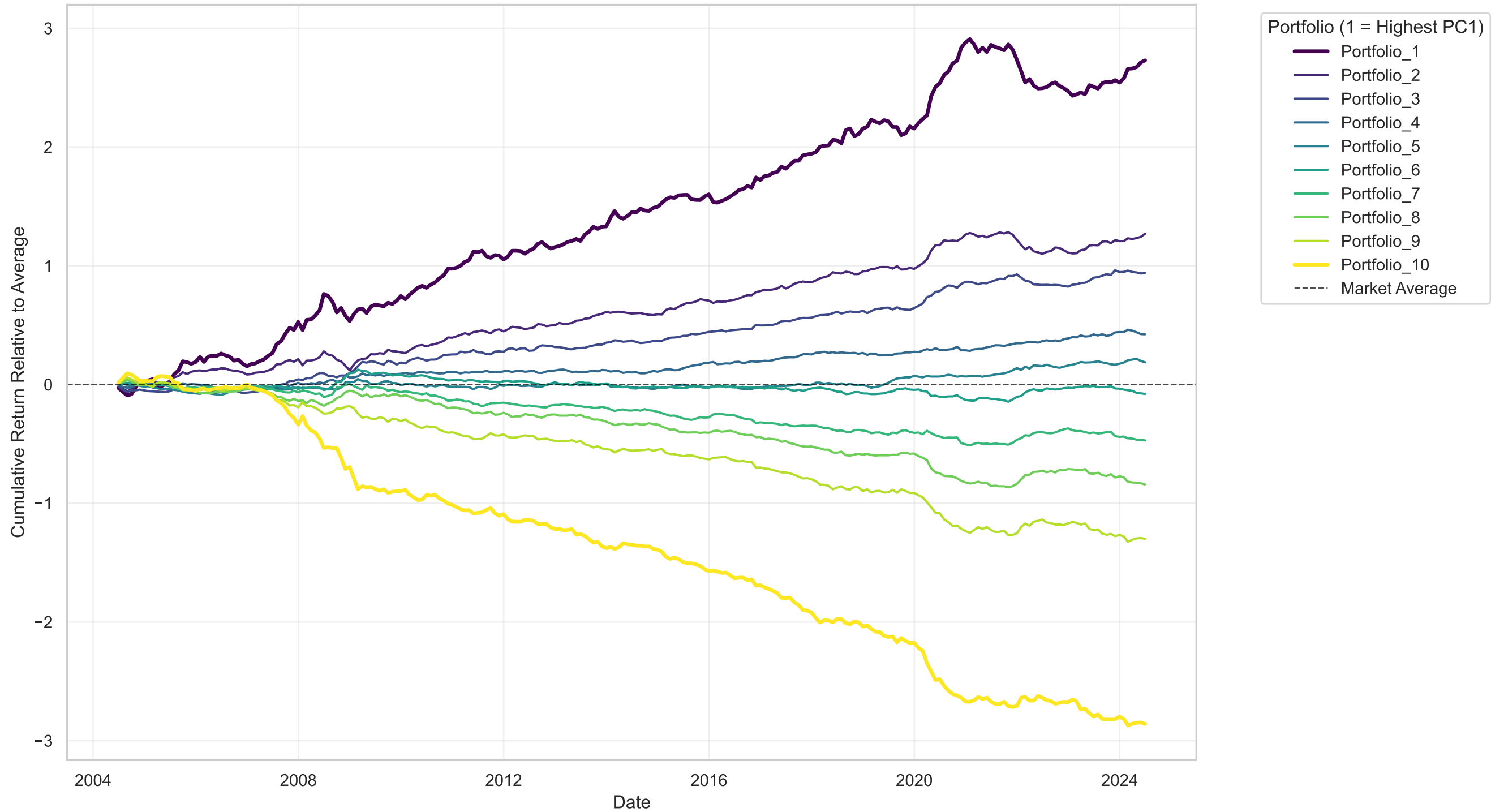
Cumulative Relative Returns: PC1-Sorted vs. Market Average
