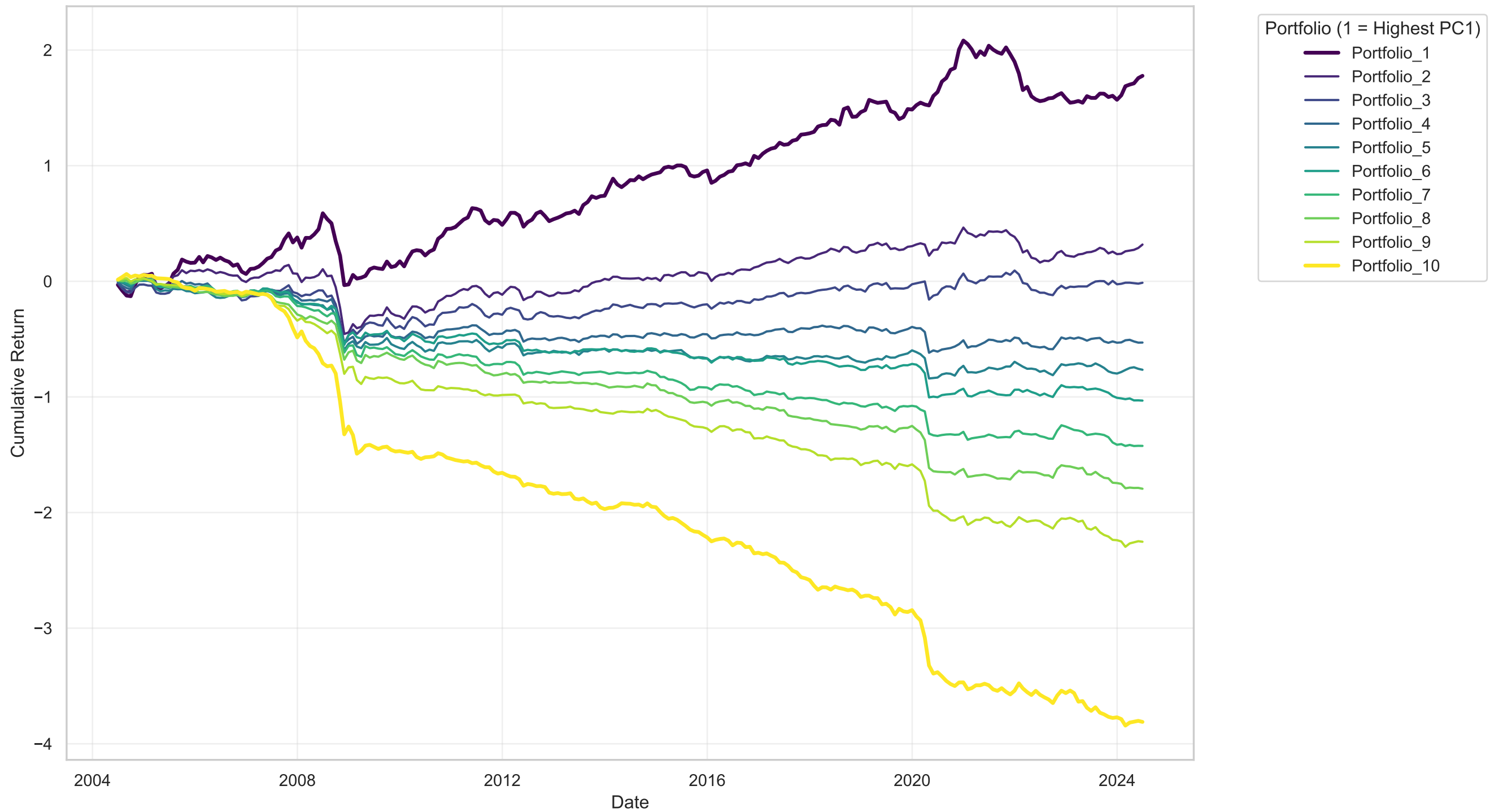
Cumulative Returns: PC1-Sorted Portfolios
