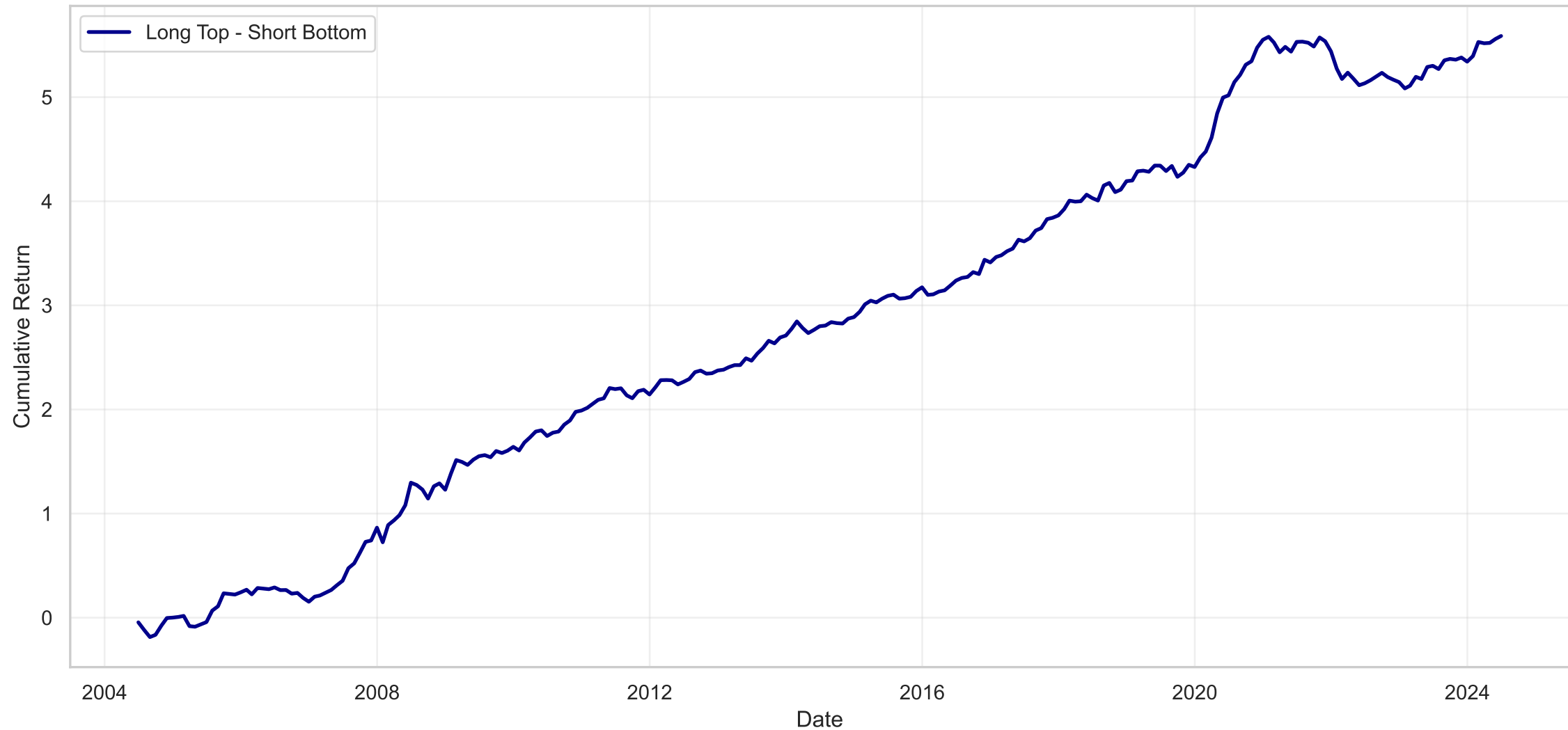
Cumulative Long-Short Portfolio Return (PC1-Sorted)
