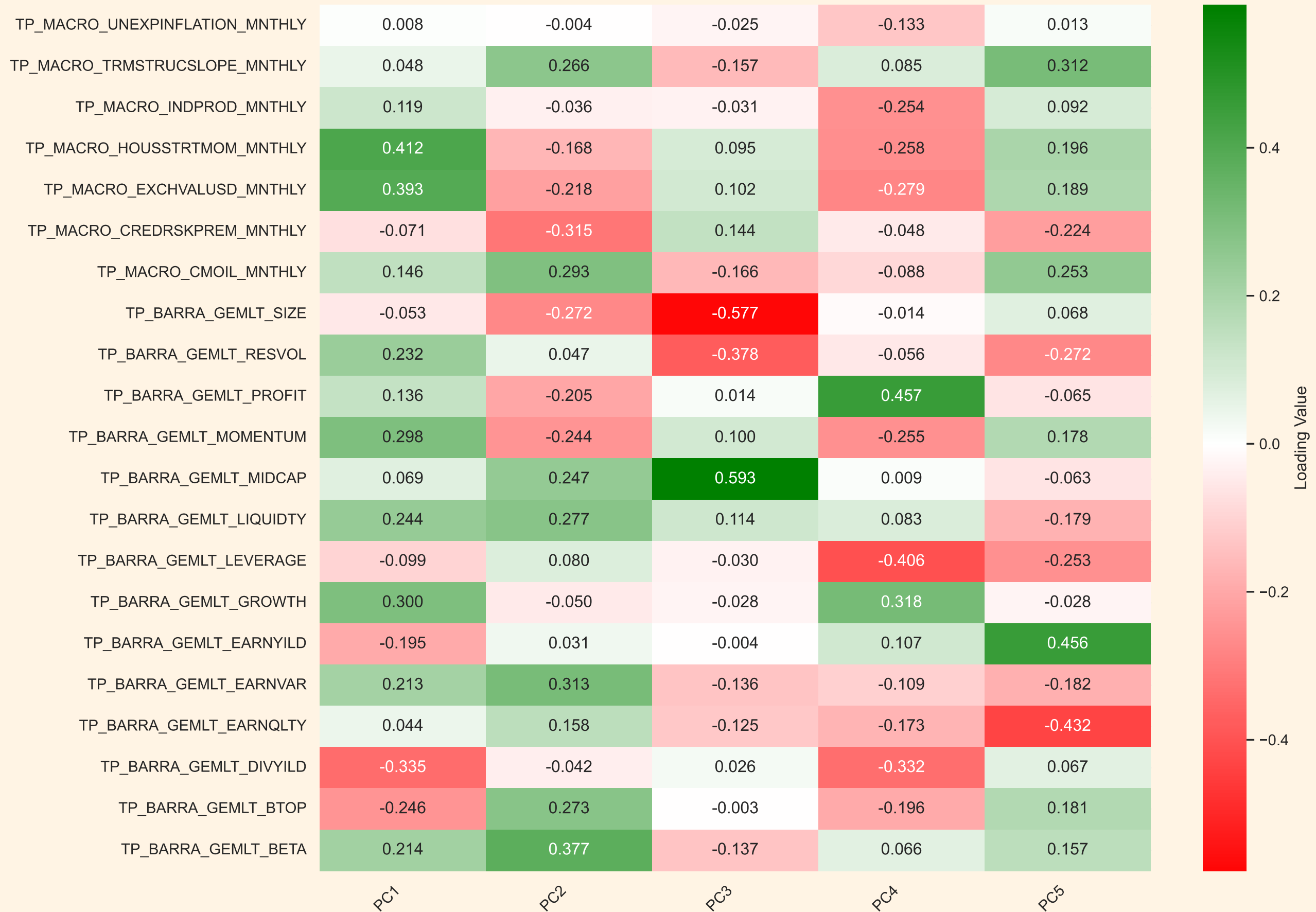
PCA Component Loadings
