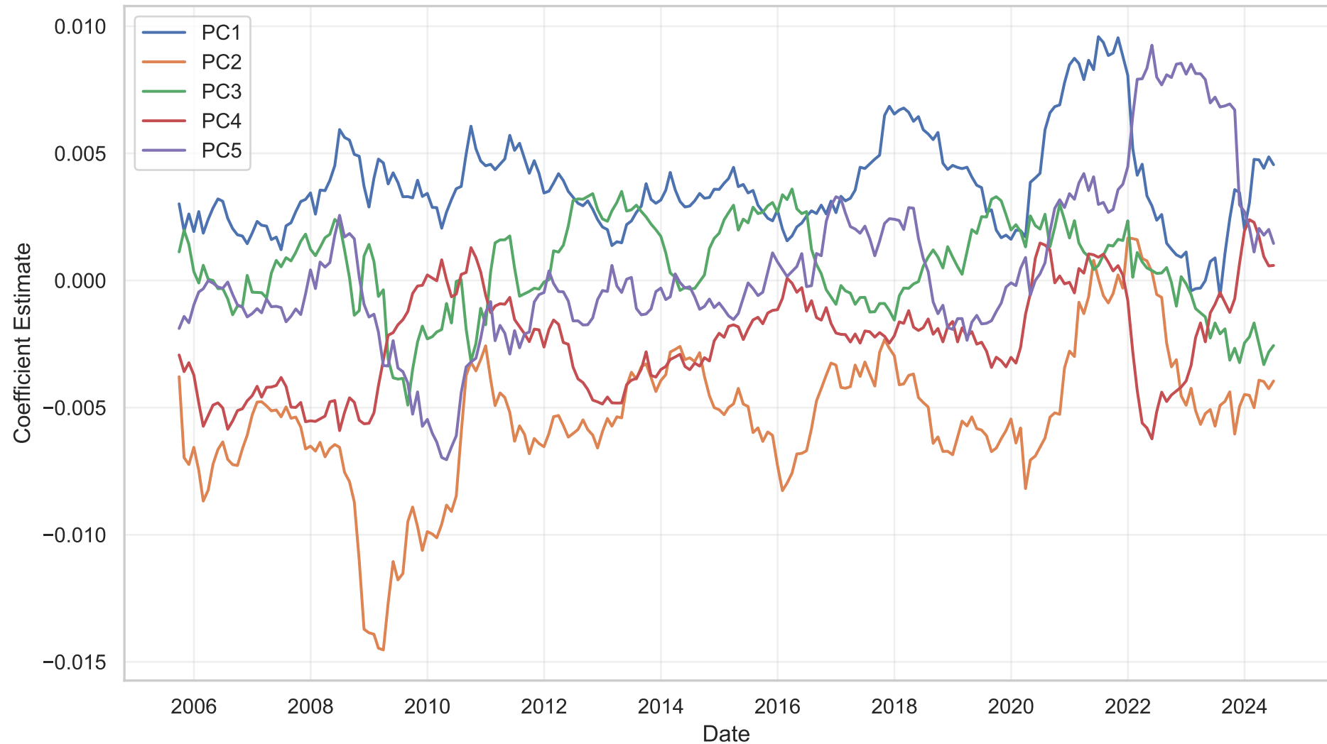
Rolling Average of Daily Regression Coefficients
